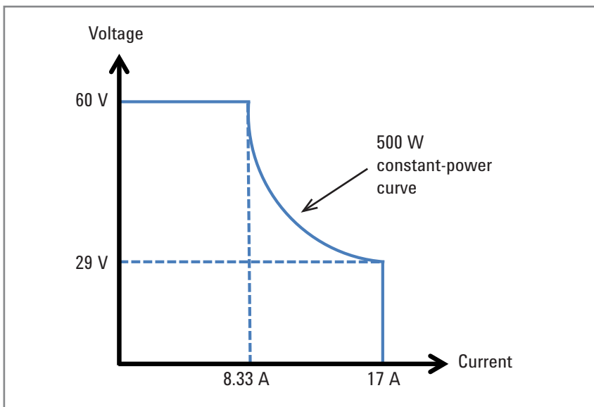
Figure 1. Autoranging output characteristic
