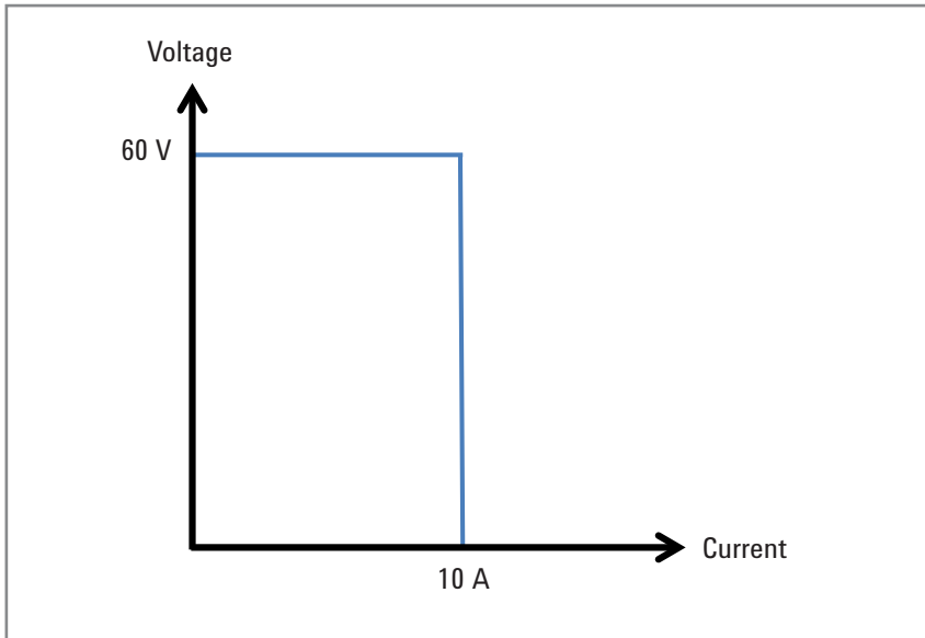
Figure 2. Rectangular Output Characteristic Voltage
